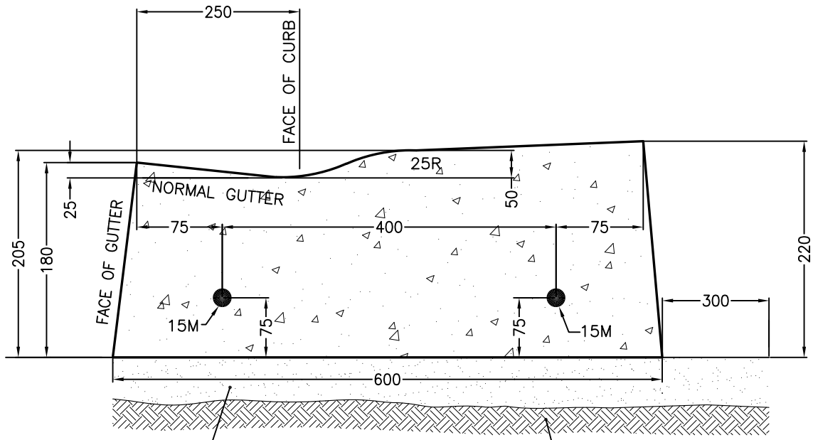
CROSSING SECTION
