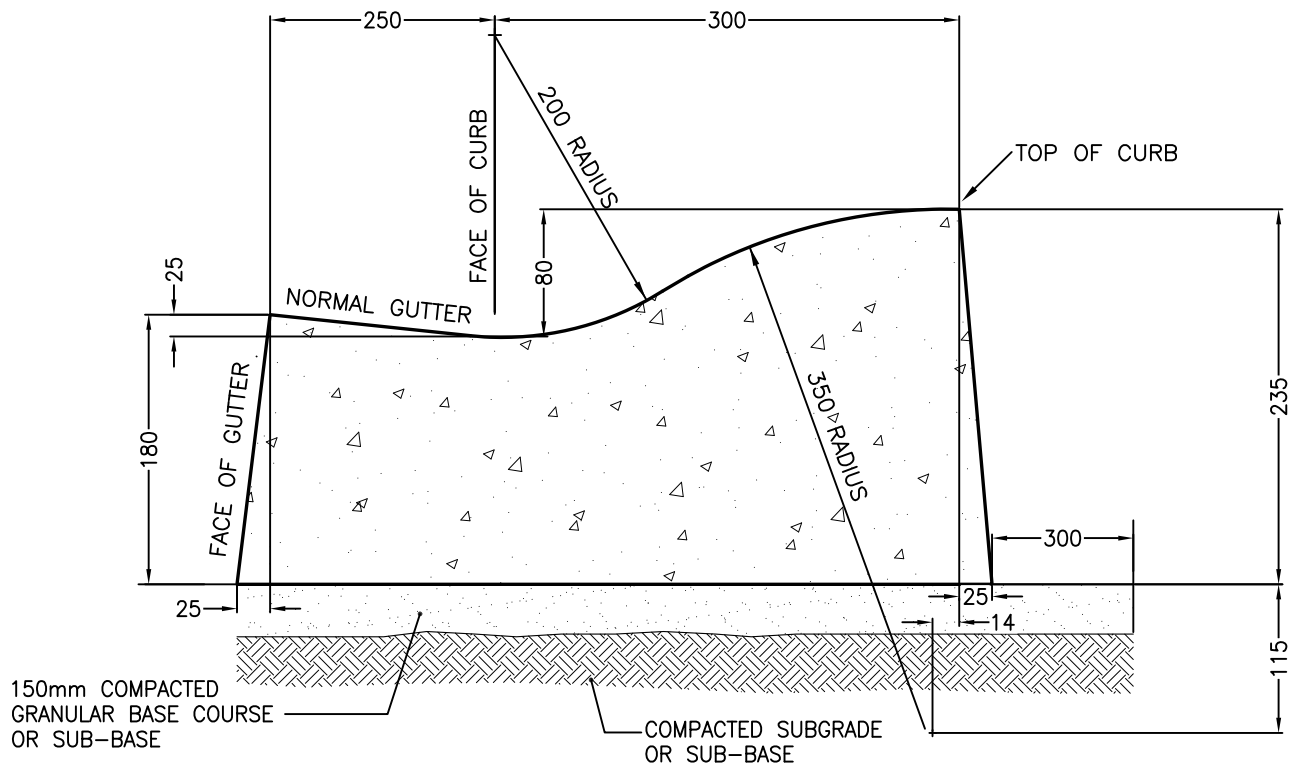
TYPICAL ROLLED CURB & GUTTER
