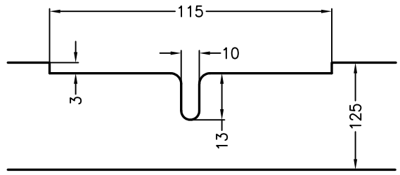
SURFACE JOINT DETAIL 'B' N.T.S
