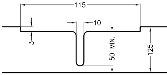
CONTRACTION JOINT DETAIL 'A' N.T.S
