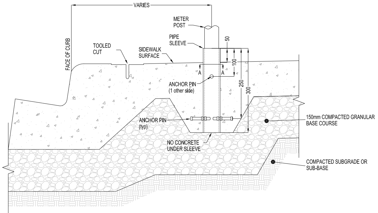
POST AND SLEEVE INSTALLATION
