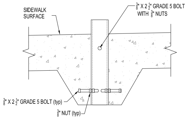
SLEEVE DETAIL
