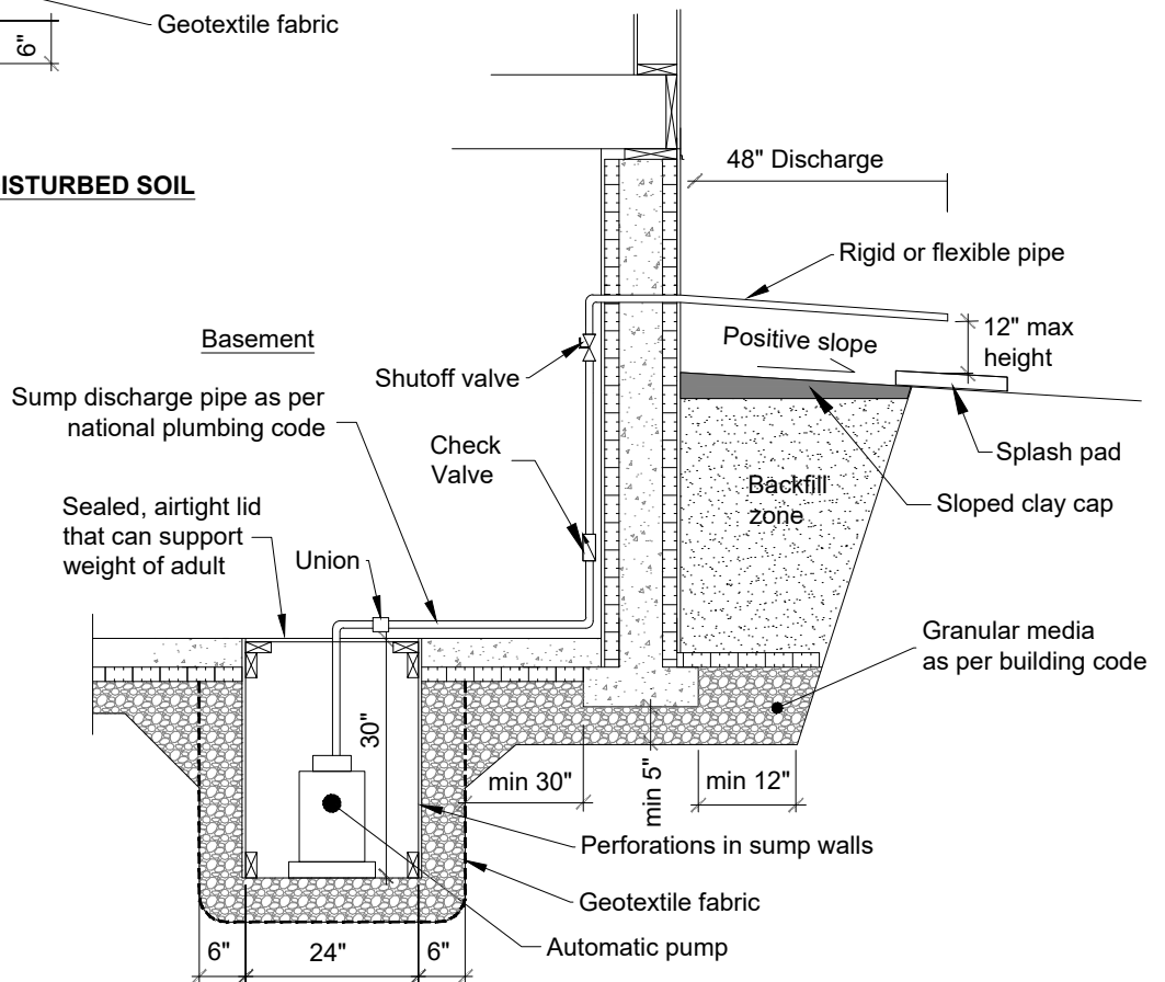
FOOTING OVER GRANULAR DRAINAGE LAYER
